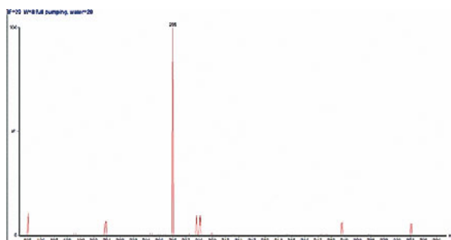
Fig. 4. PADI-MS spectra of an ibuprofen tablet using 8 W plasma power, 2 mm distance, and 284 m/min helium flow rate
